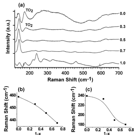
FIG. 3. (a) Room temperature Raman spectra for \text{Ca}_x\text{Sr}_{1-x}\text{TiO}_3 nanocubes. [(b) and (c)] Plots depicting the peak position of structural modes identified in each with increasing Sr concentration. The \text{TO}_2 mode is marked for the x=0 and 0.3 samples.
