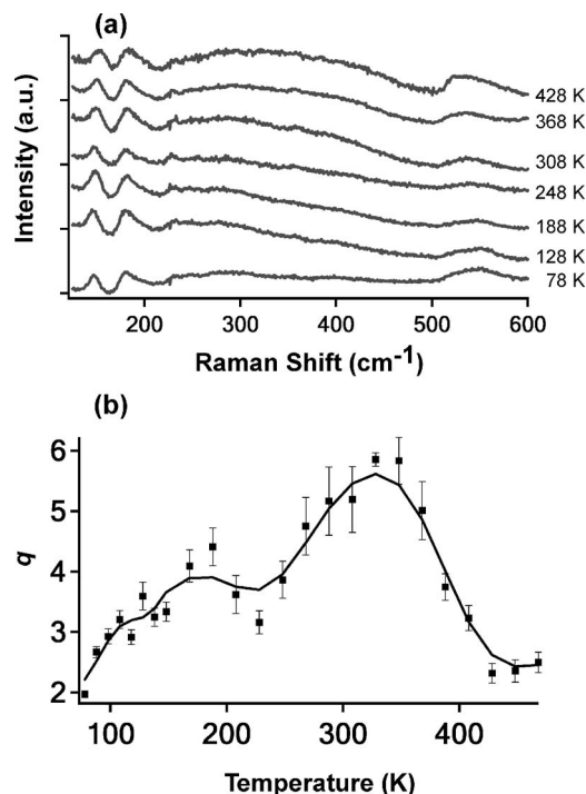
FIG. 2. (a) Representative Raman spectra obtained at different temperatures for \text{SrTiO}_3 nanocubes. The temperature was controlled within \pm 1^\circ\text{C} using a Linkam TMS 600 stage. (b) Temperature dependence of the asymmetry parameter q as obtained by fitting the Fano profiles to Eq. (1).
